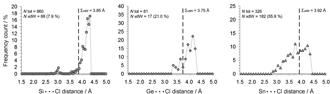
Figure 7. Plots of the frequency count [%] as a function of the R 3 Tr...Cl distance [Å] for Tr = Si (a), Ge (b), and Sn (c). The solid lines are added as a guide to the eye and the vertical dashed lines indicate the sum of the van der Waals radii of Tr and Cl. The inset numbers represent the total amount of data ( N_{\text{tot}} ) and the absolute and relative amount of data displaying van der Waals overlap.
